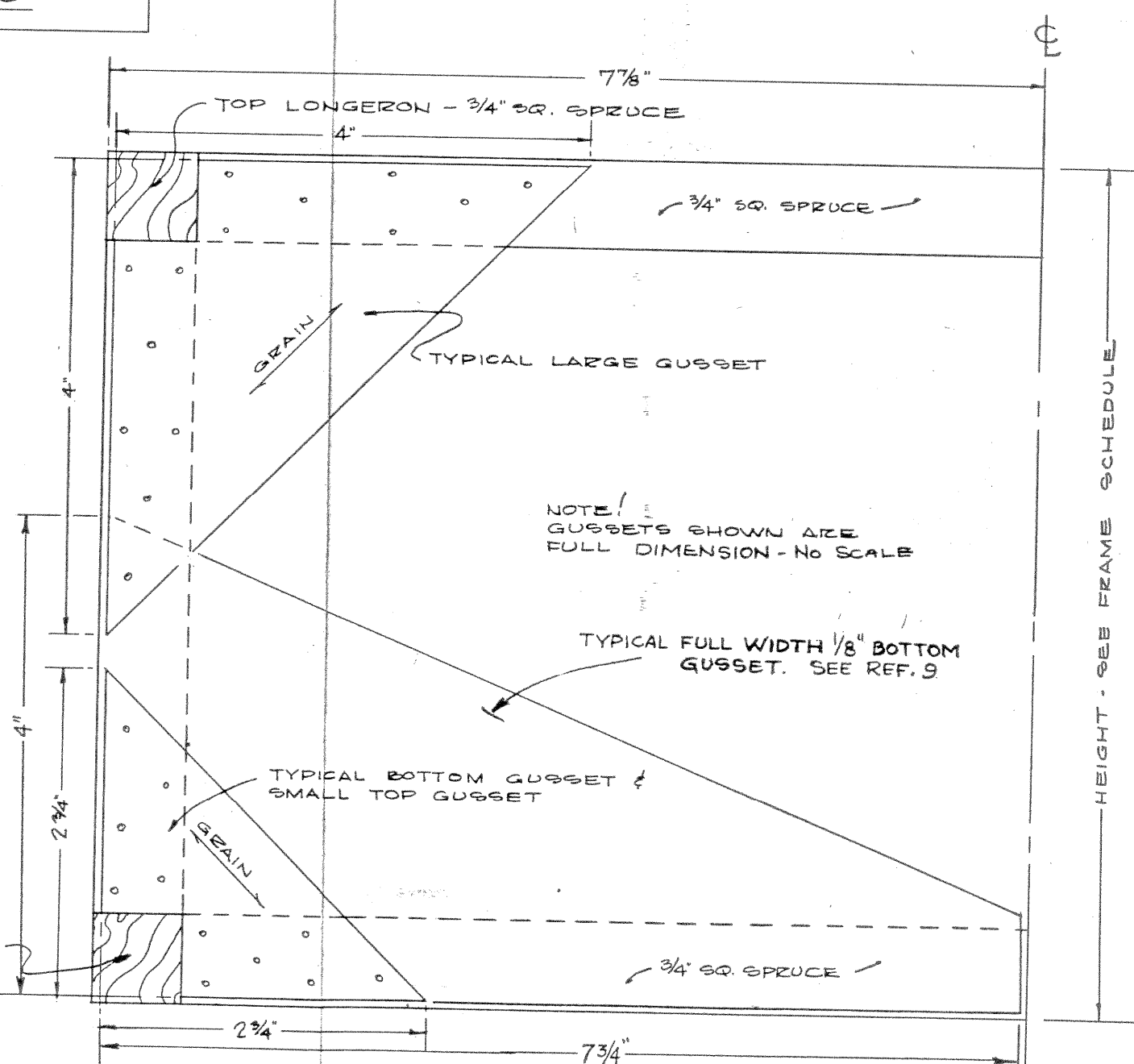
TYPICAL FRAME DETAIL (ONLY ONE-HALF OF FRAME SHOWN)
