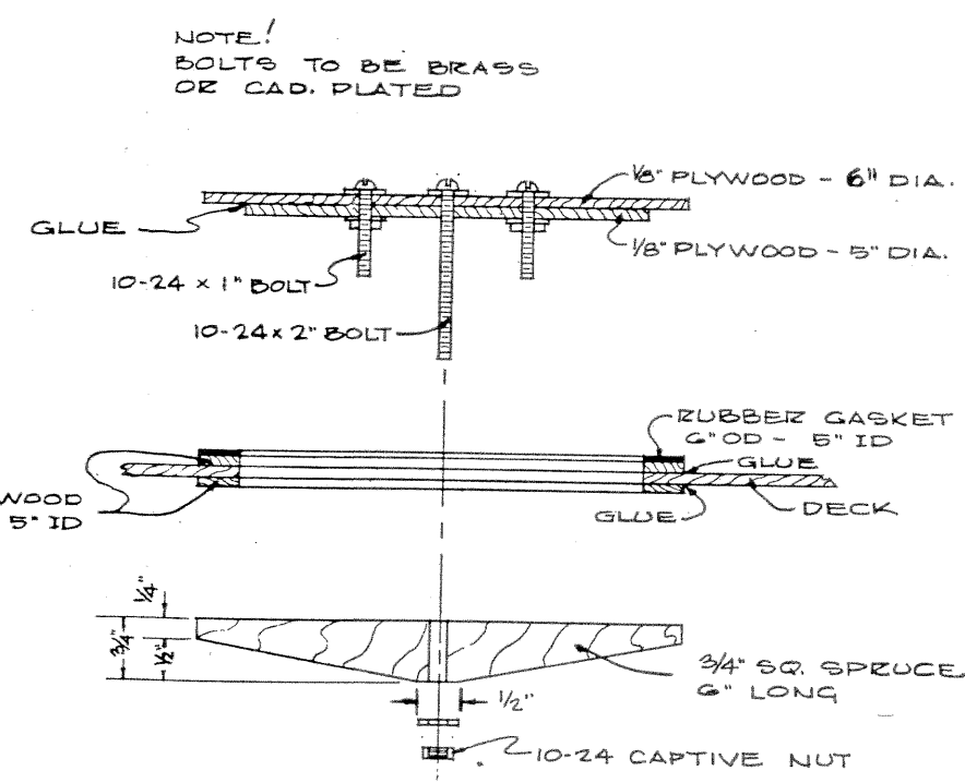
SECTION HAND HOLE DETAIL
