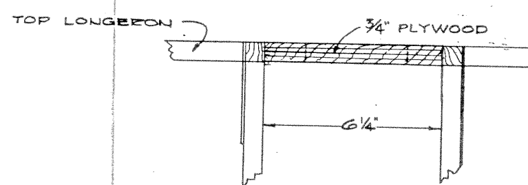
MOUNT PLATE DETAIL SECTION 1-1
