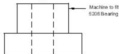
Bottom Bearing Bushing
