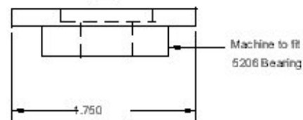
Top Bearing Bushing
