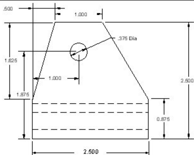
Bottom Bearing Bushing
