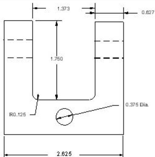
Top Bearing Bushing
